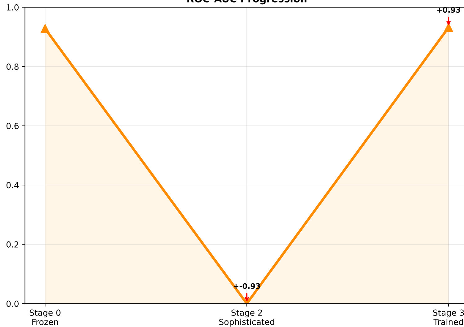
ROC-AUC Progression
